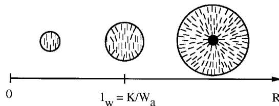
Figure 1. Schematic structures of nematic droplets with normal anchoring. Large droplets with R \gg K/W_a contain topological defects in equilibrium; in small droplets with R \ll K/W_a the director tends to be uniform.
