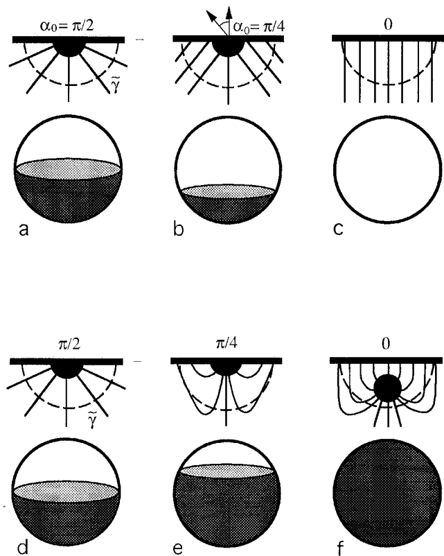
Figure 5. Two possible ways of boojum transformation under changing boundary conditions. The scenario (a, b, c) results in gradual disappearance of the defect, while the scenario (d, e, f) produces a point defect hedgehog. The corresponding characteristics A are shown as the shadowed areas on a sphere of the order parameter space below each boojum structure.
